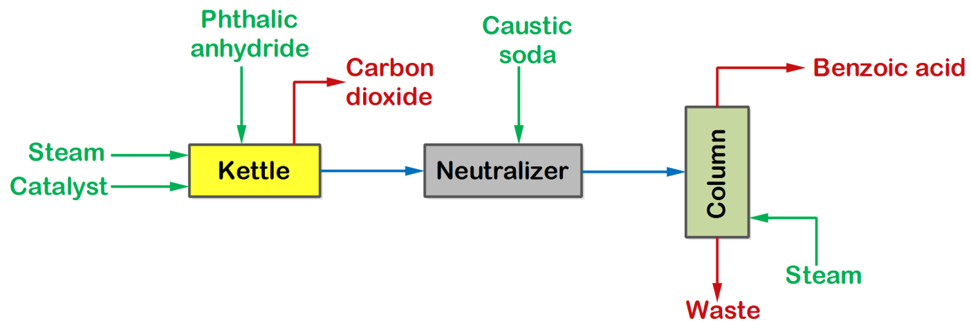
Figure: Manufacture of Benzoic acid from Phthalic anhydride
